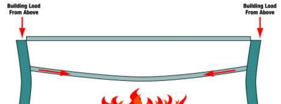
Figure 2-21 Buckling of columns initiated by failure of floor framing and connections.
